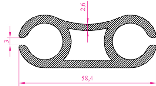
Profil N o :2585 Ag ırık 1,428 kg/m
